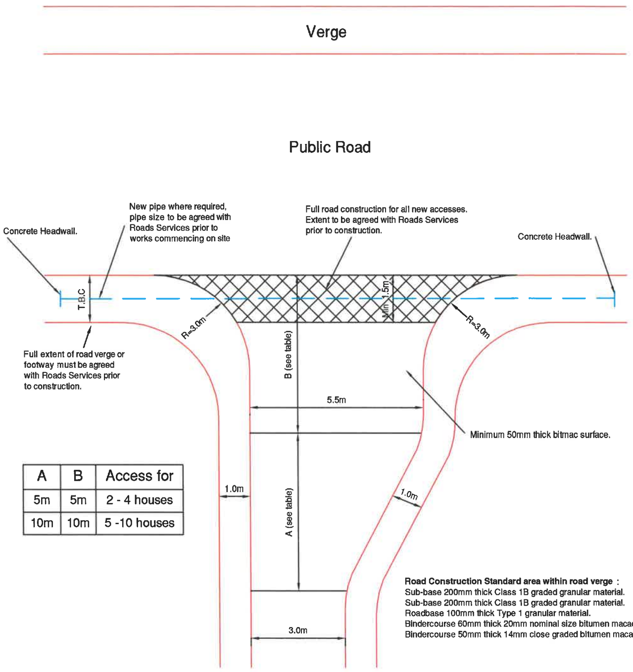
TYPICAL ACCESS FOR SINGLE DEVELOPMENT (NON-ADOPTED)
